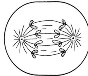
Anaphase
