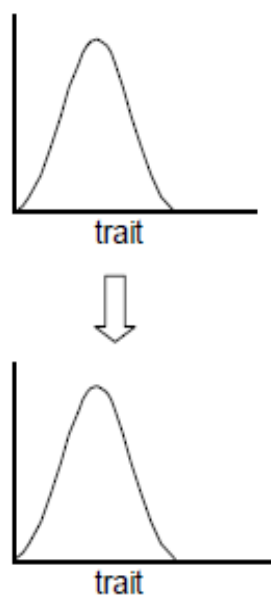
Stabilising Selection
