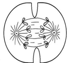
Telophase
