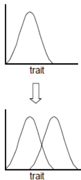
Disruptive Selection
