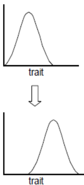
Directional Selection
