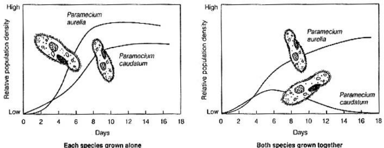
Figure 6-3 The results of G. F. Gause's classic laboratory experiment with two similar single-celled, bacteria-eating species of Paramecium (that reproduce asexually) support the competitive exclusion principle that similar species cannot indefinitely occupy the same ecological niche.
